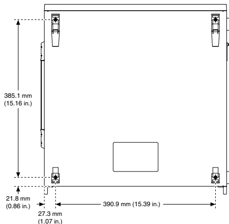
Figure 2. PXIe-1084 Chassis Dimensions (Bottom)
